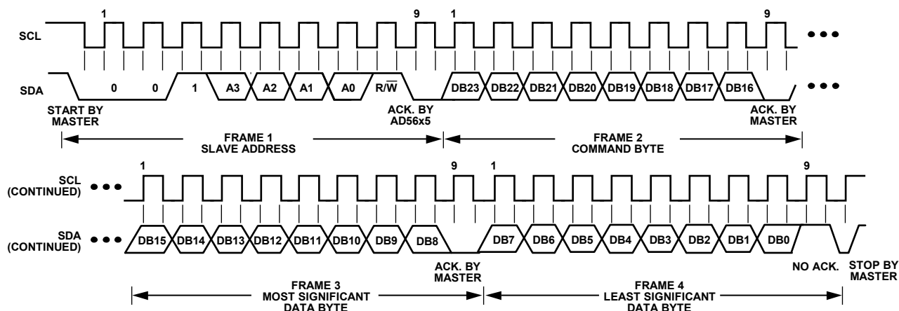
Figure 60. I 2 C Read Operation (14-Lead Package)
