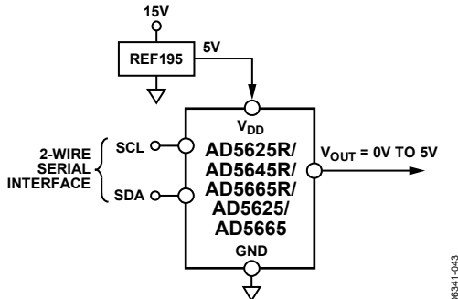
Figure 72. REF195 as Power Supply to the AD56x5R/AD56x5
